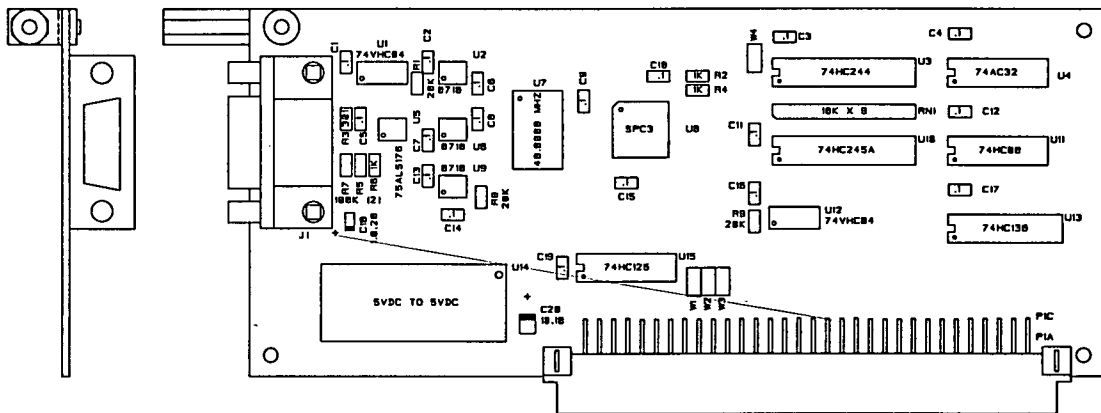
PROFIBUS-DP INTERFACE BOARD FIGURE 2-1
