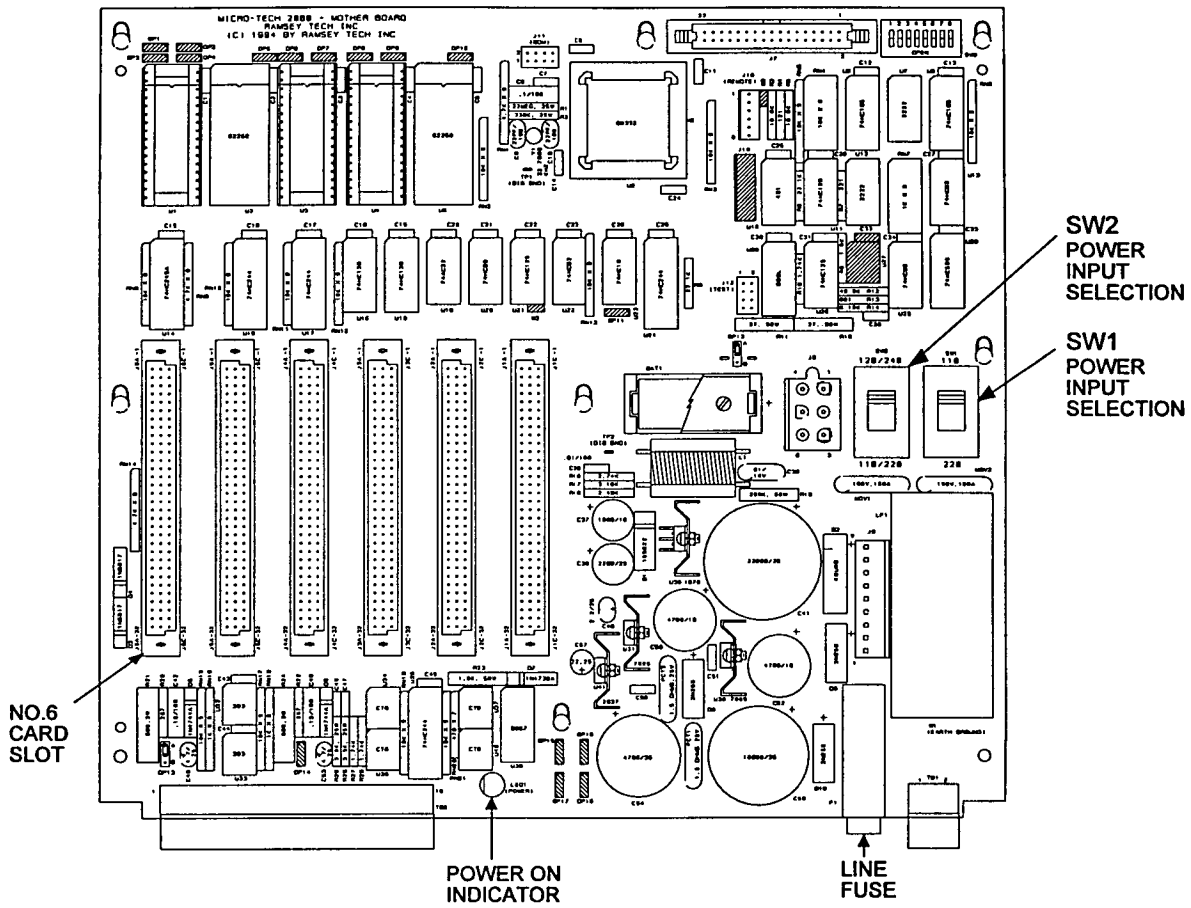
MODEL 2000 MOTHER BOARD FIGURE 2-2
